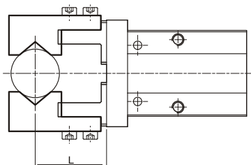
External grip
